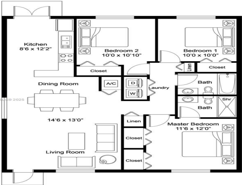
FLOOR PLAN
